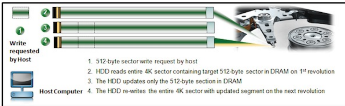
Figure 4 Alignment conditions
